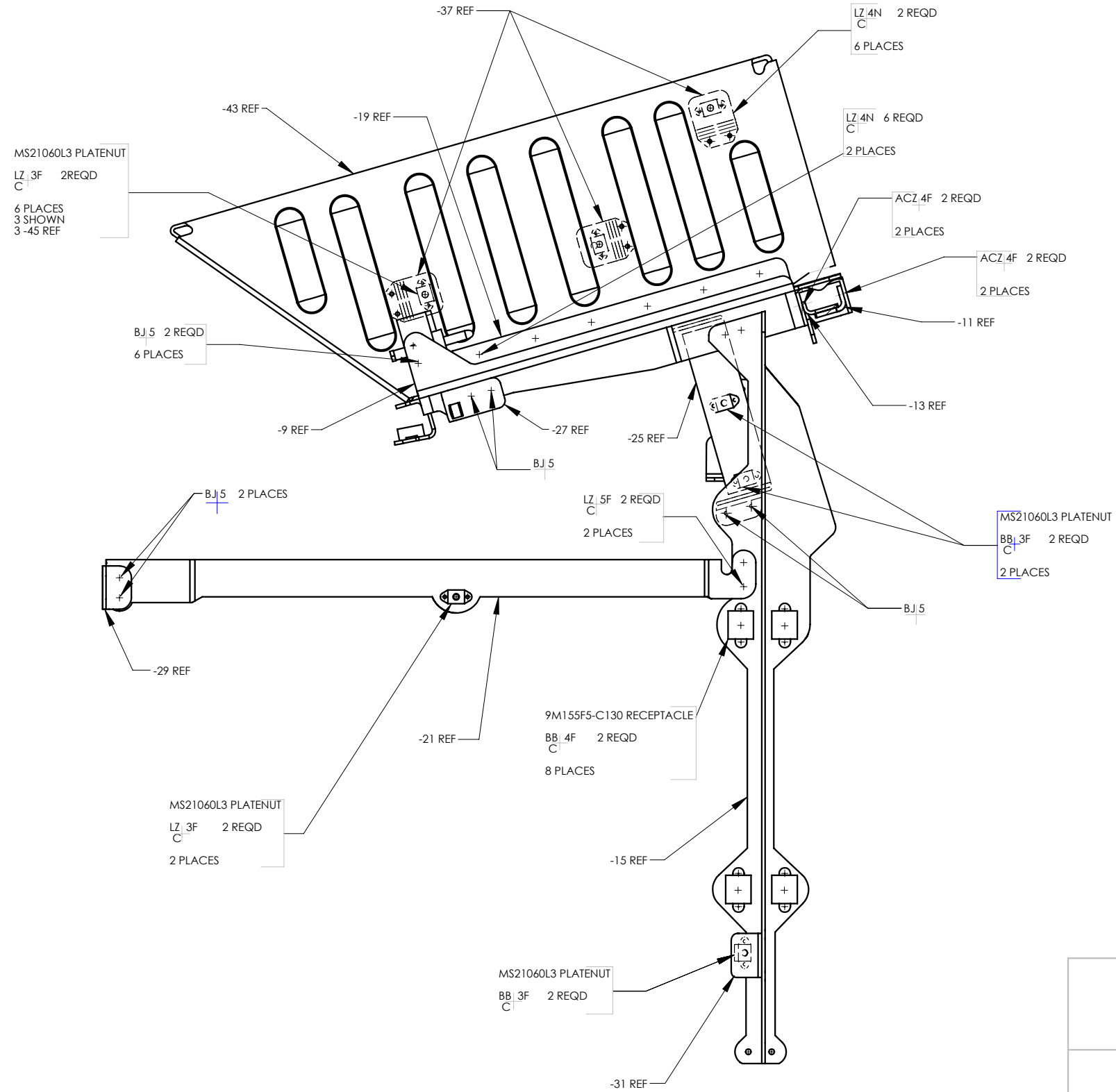
VIEW B-B ROTATED 90° CCW
