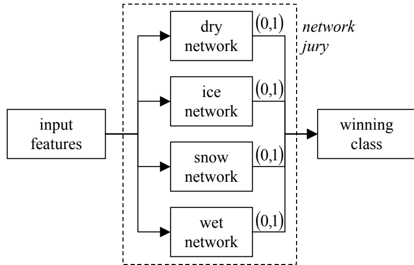
Figure 3: Diagram of neural network jury for classification.
