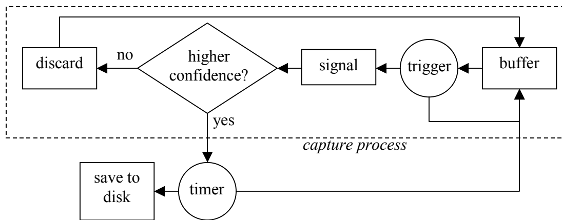
Figure 1: Capture process for acoustic signals.
