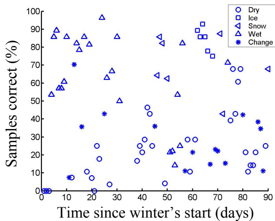
Figure 4: Classification without confidence.
